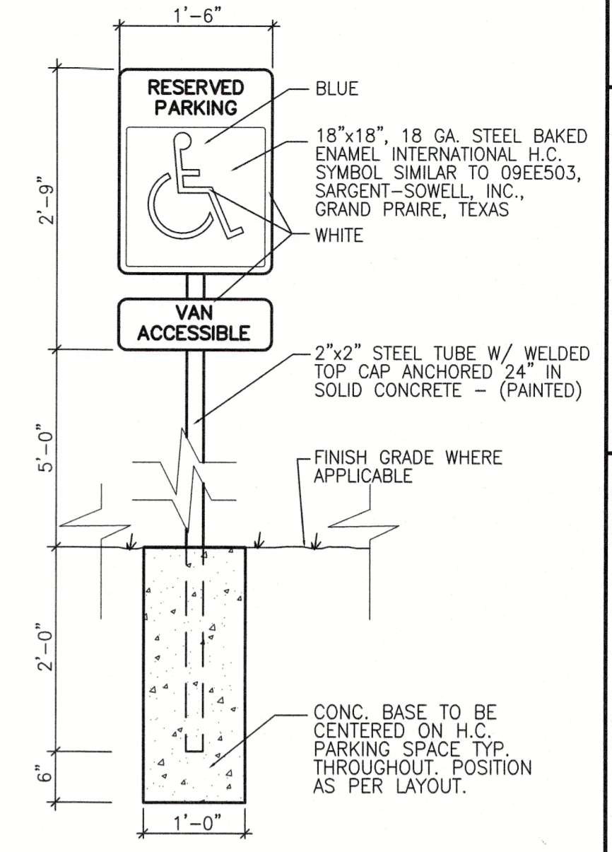
2 HC PARKING SIGN C102 3/4" = 1'-0"
